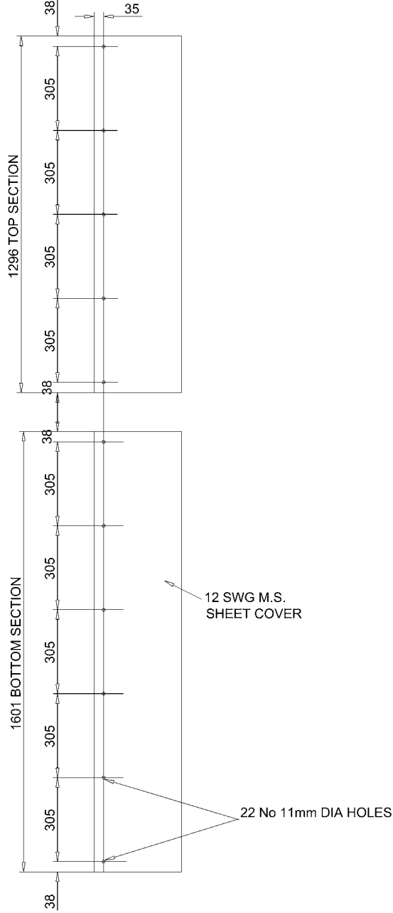
SIDE ELEVATION
