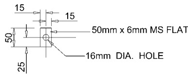
DETAIL ① 6 No REQUIRED 1:5
