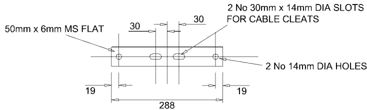
DETAIL ② 3 No REQUIRED 1:5
