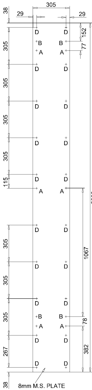
BACK PLATE DETAIL ④
